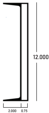
C Channel
