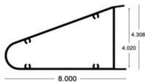
Sloped Bullnose
