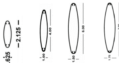
Air Foil
